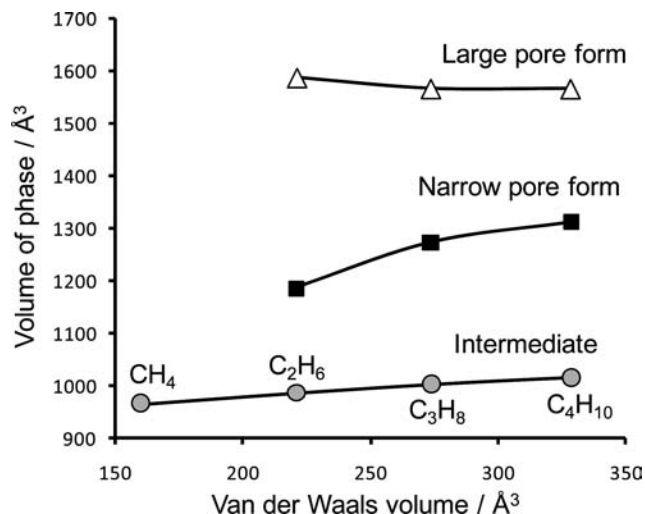
Figure 7. Unit cell volume of the various MIL-53(Fe) phases at 303 K as a function of the van der Waals volumes of the probe molecules.
