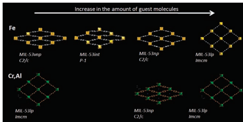
Figure 1. Structural evolution of MIL-53(Fe) (top) and MIL-53(Cr,Al) (bottom) with an increase in the amount of guest molecules inside the system (from left to right).
