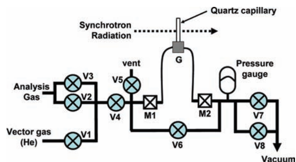
Figure 2. Schematic diagram of the dosing manifold.
