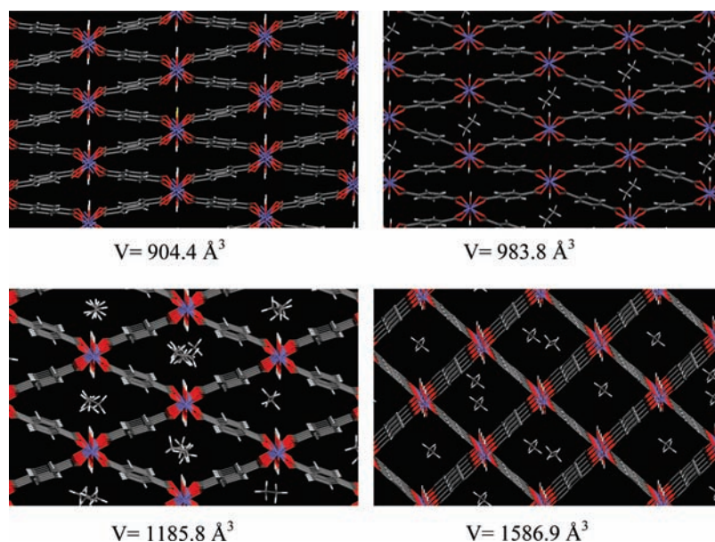
Figure 6. Illustration of the structural behavior of the MIL-53(Fe) solid upon ethane adsorption (simulated structures): very narrow pore (top left), intermediate (top right), narrow pore (bottom left), and large pore (bottom right) forms. Cell volumes are also indicated.
