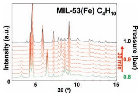
Figure 5. Kinetic evolution of the XRPD pattern of MIL-53(Fe) at 0.9 bar of butane at 303 K. The colors correspond to the major phase observed at the given pressure: green, intermediate ; red, narrow pore ; black, large pore form.
