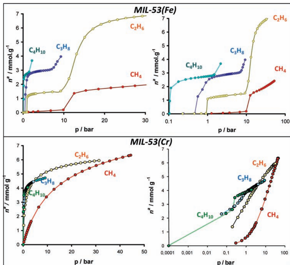
Figure 3. Adsorption isotherms of the C1–C4 linear hydrocarbons at 303 K in MIL-53(Fe) (top) and MIL-53(Cr) 19 (bottom): standard coordinates (left); semilog plot (right).
