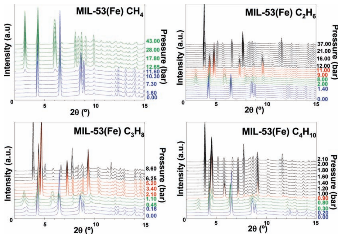
Figure 4. Adsorption of linear alkanes on MIL-53(Fe) at 303 K followed by XRPD. The color corresponds to the major phase observed at the given pressure: blue, anhydrous very narrow pore form; green, intermediate form; red, narrow pore form; black, large pore form.
