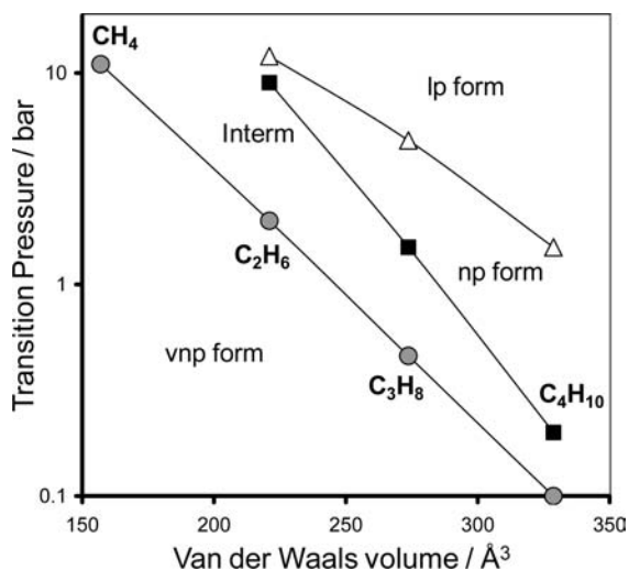
Figure 8. Variation of the transition pressures of MIL-53(Fe) at 303 K as a function of the van der Waals volumes of the alkane molecules.
